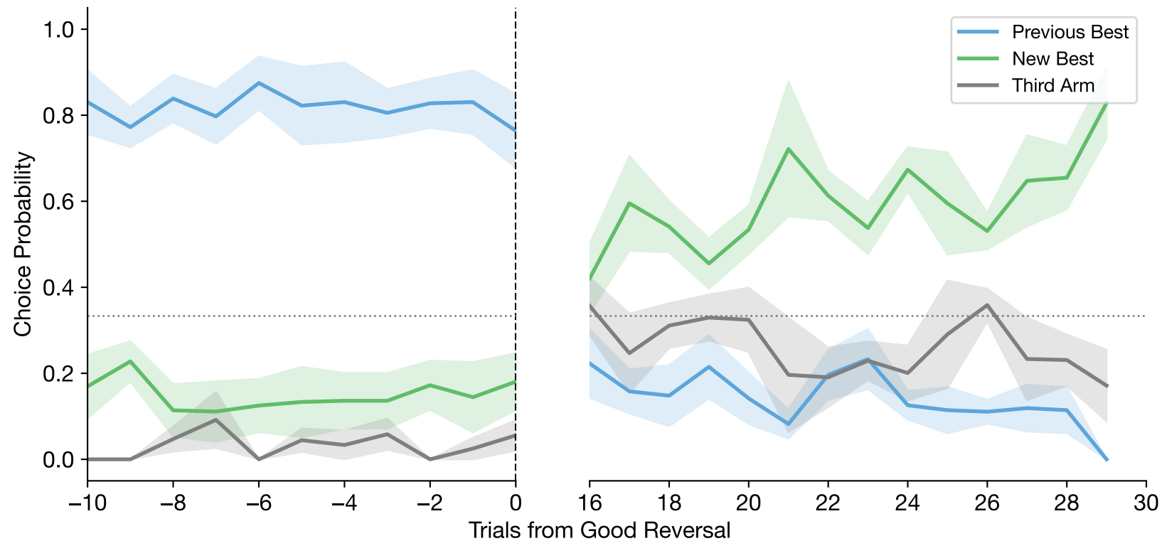
Good Reversal-Aligned Choices (mean \pm se across subjects | n=5 subjects, n=40 reversals) (Skipping first 15 trials post-reversal)
